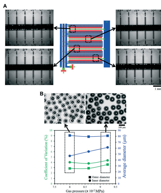
Fig. 4 Mass production of monodisperse compound bubbles in microfluidic device. (A) Representative optical images illustrating uniform generation of G/W/O compound bubble in 400 parallelized FFGs. A movie illustrating the production of G/W/O compound bubbles is provided in the ESI. (B) Change of compound bubble size and coefficient of variation as gas pressure generated in 400-FFGs.
