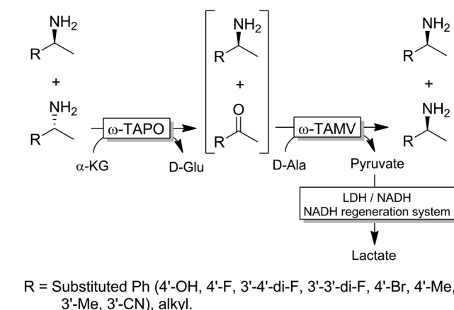
Scheme 19 One pot deracemisation via stereoinversion of amines using two orthogonal (with respect to the preferred amine-donor or acceptor) and enantiocomplementary \omega -TAs. TAPO: \omega -transaminase from Polaromonas sp., TAMV: \omega -transaminase from Mycobacterium vanbaalenii (EC 2.6.1.18), LDH: lactate dehydrogenase (EC 1.1.1.27).
