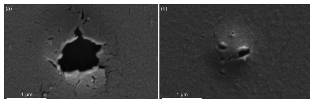
Fig. 2 Single Ag layer (50 nm, on glass). Scanning electron micrographs of microbump breaching. F_{\text{inc}} = 2.11 \text{ J cm}^{-2} , F_{\text{abs}} = 0.25 \text{ J cm}^{-2} , N = 1 , w = 1.40 \pm 0.06 \text{ μm} .
