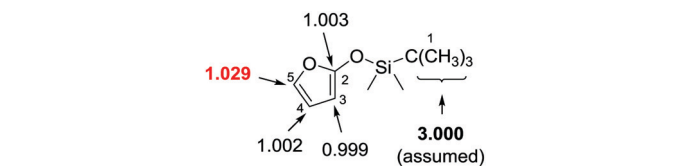
Scheme 11 Carbon isotope effects (R/R 0 ) calculated for TBSOF furan. The three methyl carbons of the tBu group (in bold) were taken as the internal standard.
