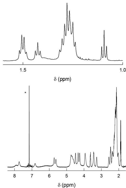
Fig. 6 ^1\text{H} NMR spectrum of 1 mM \text{Au}_{144}(\text{SC}_3)_{60} in \text{C}_6\text{D}_6 at 25 °C. For convenience, the spectrum has been divided into two parts: \gamma\text{-CH}_3 (top) and \alpha\text{-CH}_2 and \beta\text{-CH}_2 (bottom). In the latter, the scale has been enlarged (6.3 \times ). The asterisk marks the benzene signal.
