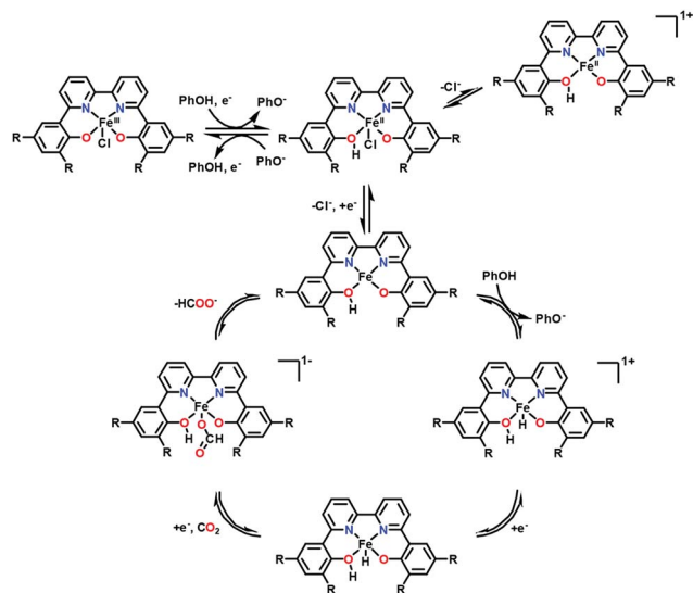
Scheme 8 Catalytic cycle for two-electron reduction of \text{CO}_2 to CO with a nonheme iron(III) chloride complex bearing a 6,6'-di(3,5-di- tert -butyl-2-hydroxybenzene)-2,2'-bipyridine ligand ( \text{Fe}^{\text{III}}(\text{t}^{\text{bu}}\text{dhbpy})\text{Cl} ) via protonation by phenol. Reprinted with permission from ref. 127. Copyright 2018, American Chemical Society.
