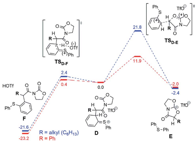
Fig. 7 Computed reaction profile (DFT, \Delta G_{298, \text{DCM}} ) for the conversion of the intermediate D into the main product F or the bicyclic cation E for the phenyl (red) and the alkyl (blue) substrates. The energy of the intermediate D is taken as a reference (0.0 kcal mol -1 ).
