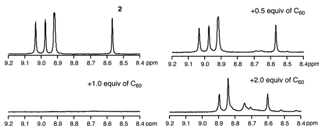
Fig. 7 1 H NMR spectra of 2 and 2 + C 60 at −40 °C in toluene- d 8 .
