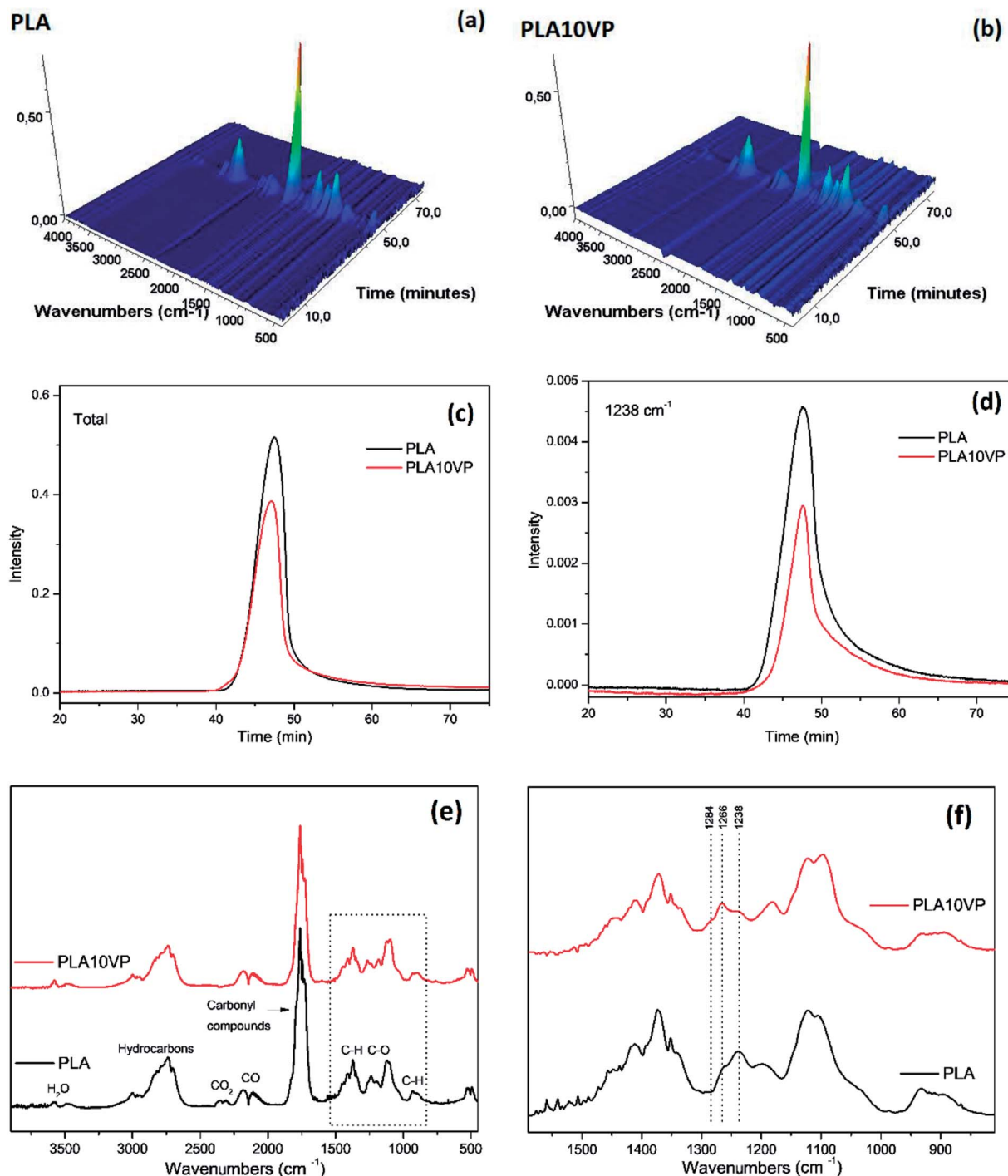
Fig. 7 3D-images of evolved gaseous products for (a) PLA (b) PLA10VP; (c) total absorbance vs. time for PLA and PLA10VP; (d) absorbance at 1238 cm -1 vs. time for PLA and PLA10VP (e) at T_{max} for PLA and PLA10VP; (f) zoom in on selected area. ( T_{max} appeared at 47 min).
