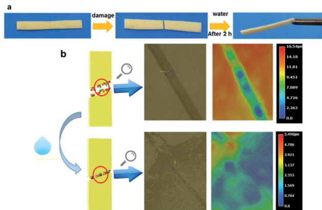
Fig. 9 Self-healing of PVP/p(HEMA-co-BA) material: (a) self-healing process of the material; (b) 3D ultra-depth of focus images of the material before and after self-healing.
