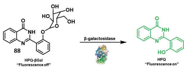
Scheme 77 An AIE + ES IPT fluorescent probe 88 that allows for the monitoring of β-galactosidase activity in live cells. Measurement conditions: PBS buffer (5 mM, pH = 7.3). Adapted with permission from ( Dyes Pigm. , 2018, 156 , 100–107). Copyright (2018) Elsevier.
