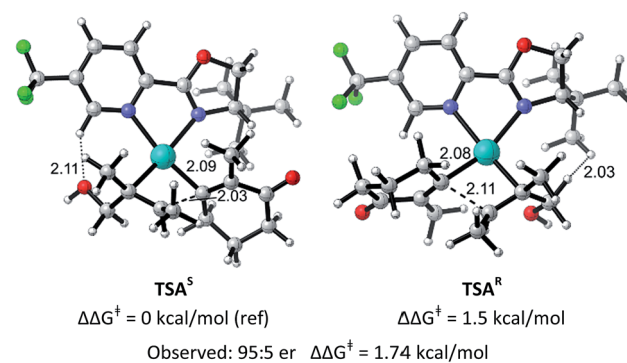
B. Lowest Energy Transition States for Alkenol 2aa
