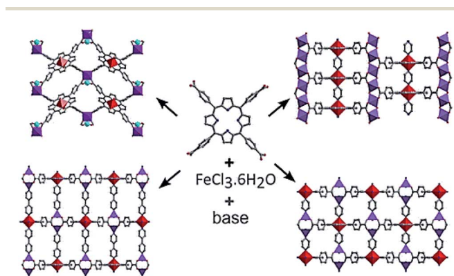
Scheme 16 The CPs obtained by the solvothermal reaction of \text{Fe}(\text{III}) chloride with tetrakis(4-carboxyphenyl)-Pp in the presence of different bases. [Reprinted with permission from ref. 212. Copyright 2015, American Chemical Society.]
