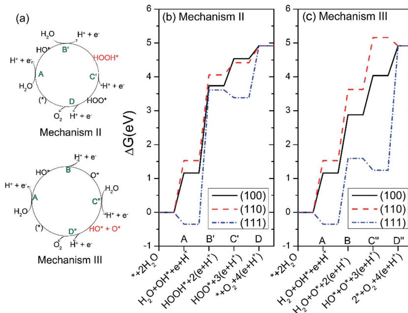
Fig. 6 (a) Oxygen evolution reaction (OER) mechanism II and III. (b and c) The free energies of the intermediates on Ag 3 PO 4 (100), (110) and (111) surfaces following mechanism II (b) and III (c) at pH = 0 and U = 0 .
