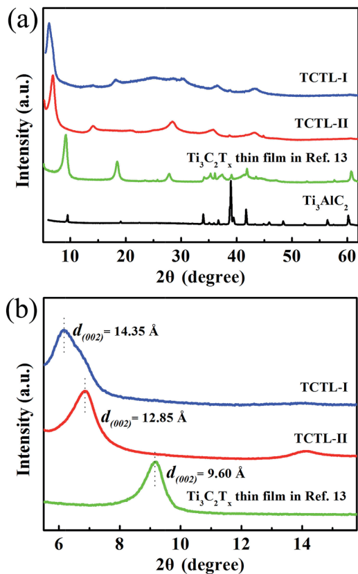
Fig. 2 (a) XRD patterns of the TCTL-I, TCTL-II, the previous Ti 3 C 2 T x thin film in ref. 13, and Ti 3 AlC 2 powder and (b) the corresponding enlarged XRD patterns.
