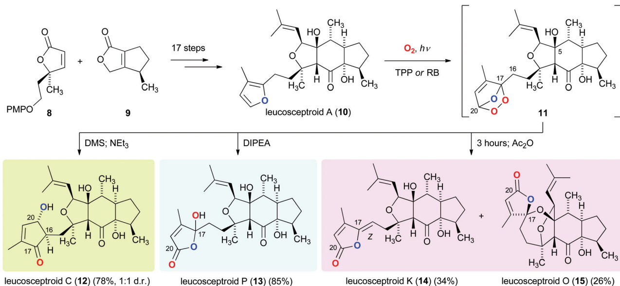
Scheme 2 Photo-oxidation of leucosceptroid A (10) for the bioinspired total synthesis of leucosceptroids C (12), P (13), K (14), and O (15).
