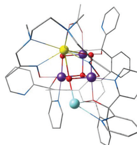
Fig. 12 \text{Mn}_3\text{CaO}_4 -Ag complex by Kanady et al. 181
