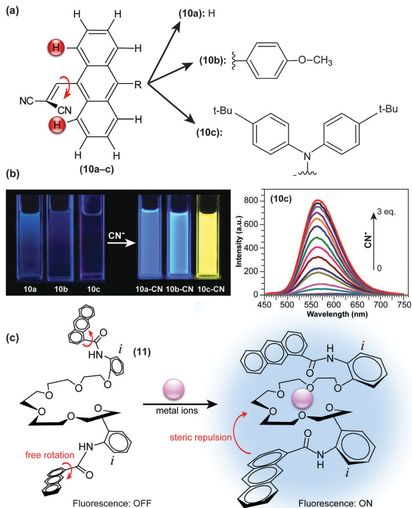
Fig. 5 (a) Chemical structures of "turn-on" \text{CN}^- probes (9-dicyanovinyl anthracene) with various functional groups ( 10a–10c ). (b) Fluorescence emission of 40 \mu\text{M} of compounds 10a–c under UV excitation with a portable lamp in the absence and presence of 3 eq. \text{CN}^- . Right: Fluorescence changes upon addition of \text{CN}^- to 10c (20 \mu\text{M} , \lambda_{\text{ex}} = 396 nm) in \text{CH}_2\text{Cl}_2 . (c) Proposed structural change of N,N -(ethylenedioxybis(3-oxapentamethyleneoxy-2-phenyl))-bis(1-anthracenecarboxamide) in response to metal ions in the ground state. Adapted from ref. 38, 42 with permission from the Royal Society of Chemistry ©2013 and the Japan Society for Analytical Chemistry ©2009.
