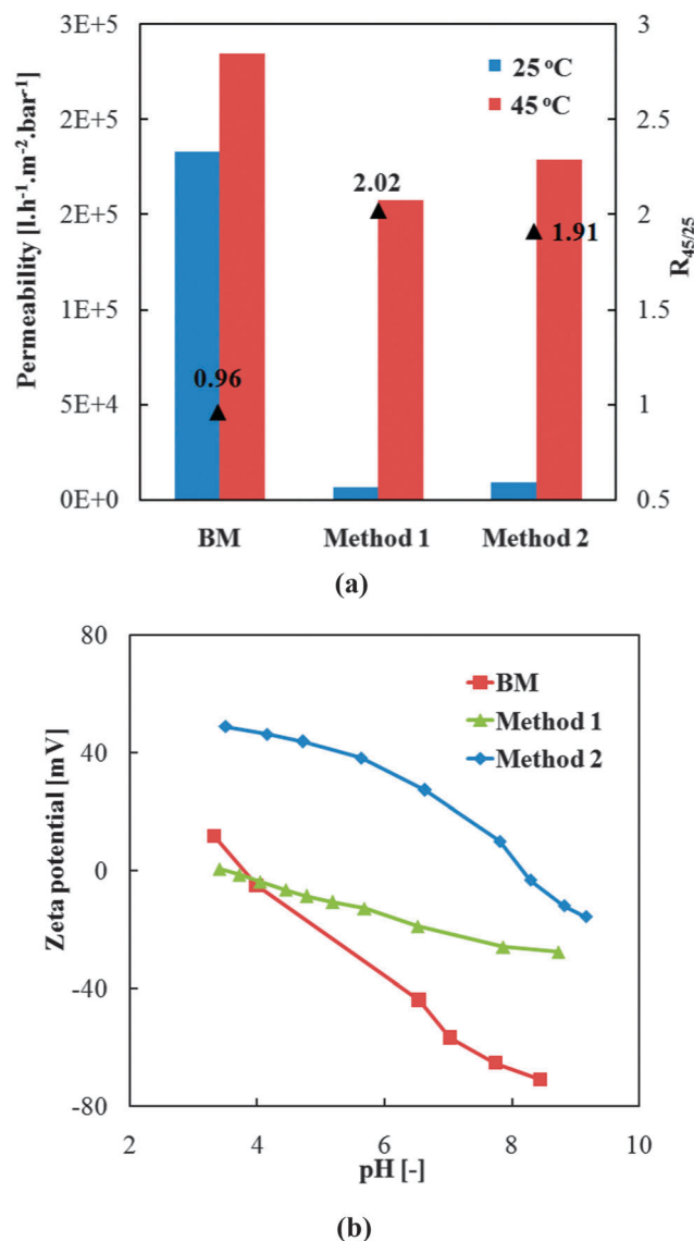
Fig. 6 Thermo-responsivity of water flux (a) and zeta potential (b) of pre-modified PET track-etched membranes obtained by methods 1 and 2 (cf. Fig. 2).
