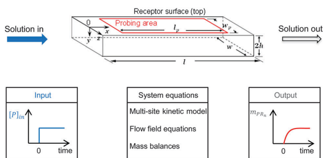
Fig. 2 Sketch of the fluid domain (upper part) and illustration of the system behavior (bottom part). The geometrical parameters are l = 2 mm, w = 0.5 mm, h = 0.01 mm, l_p = 1.8 mm, and w_p = 0.2 mm. [P]_{in} is the inlet concentration of the bionanoparticle solution. m_{PR_n}(t) is the amount of adsorbed bionanoparticles at the receptor surface.
