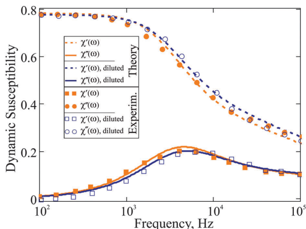
Fig. 3 Dynamic susceptibility 4\pi\chi''(\omega) of F2: comparison of the experimental data to the expressions in eqn (18). The frequency range is given on the log-scale. Here, the mass fraction of iron for the basic sample is 0.061; T = 293 K; K = 100 kJ m -3 ; effective viscosity \eta = 5 \times 10^{-3} Pa s; M_0 = 1490 kA m -1 . Reference sample: orange, filled symbols; 10 time diluted sample: blue, empty symbols (rescaled to be visible).
