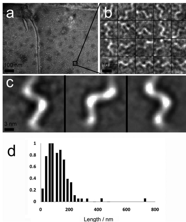
Fig. 4 (a) Contrast-enhanced TEM image showing numerous hydrogel fibrils with a twisted or helical appearance (scale bar 100 nm). (b) TEM image of a selection of twists/helical repeats in hydrogel fibrils (scale bar 10 nm). (c) Projection averages of selected images from (b), demonstrating that these repeats are regular and consistent with a helical structure (scale bar 3 nm). (d) Length distribution (normalised to highest frequency, 18, n = 118 ) of fibrils within 10 mM peptide hydrogel samples.
