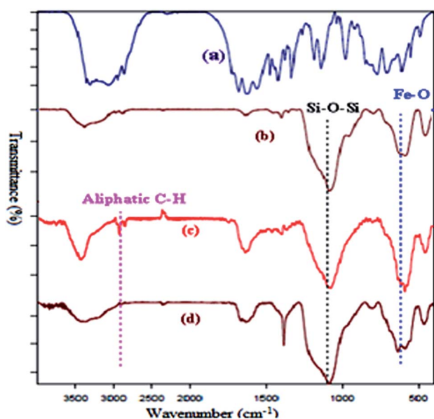
Fig. 1 FT-IR spectra of pure L-arginine (a), \text{Fe}_3\text{O}_4@ \text{SiO}_2 (b) \text{Fe}_3\text{O}_4@ \text{SiO}_2@ \text{L-arginine} (c) and \text{Cu}(\text{II}) immobilized on \text{Fe}_3\text{O}_4@ \text{SiO}_2@ \text{L-arginine} (d).
