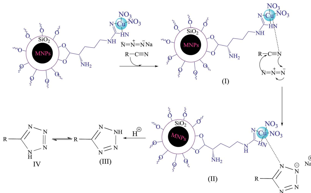
Scheme 4 Proposed mechanism for Cu(II) immobilized on \text{Fe}_3\text{O}_4@\text{SiO}_2@\text{L} -arginine catalyzed [3 + 2] cycloaddition.
