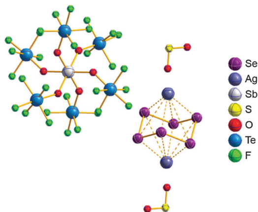
Fig. 84 Molecular structure of [(\text{SO}_2)_2\text{Ag}_2(\text{Se}_6)]^{2+}([\text{Sb}(\text{OTeF}_5)_6]^{-})_2 . D. Aris, J. Beck, A. Decken, I. Dionne, I. Krossing, J. Passmore, E. Rivard, F. Steden and X. Wang, Phosphorus, Sulfur Silicon Relat. Elem. , 2004, 179 , 859–863. Data from this reference were used to draw this figure. One anion of the formula unit and the disorder of the anion and \text{SO}_2 molecules were omitted for clarity.
