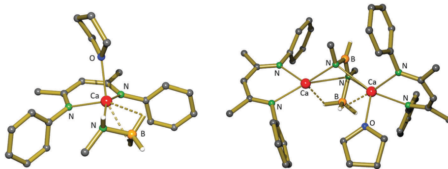
Fig. 5 Crystal structure of compound 11-Me (l) and its thermal decomposition product 12-Me (r), displaying the \text{[NMe-BH-NMe-BH}_3\text{]}^{2-} dianion. ^i\text{Pr} groups and most H atoms are omitted for clarity.
