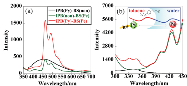
Fig. 3 (a) Fluorescence and (b) excitation spectra of the A,B-block amphiphilic polymers containing Py and Pe units dissolved in a water/toluene emulsion (118/1) including 1.8% Triton X at 25 °C, [polymer] = 0.083 g L -1 , (a) excited at 330 nm, (b) monitored at 460 nm, cell length = 1 cm.
