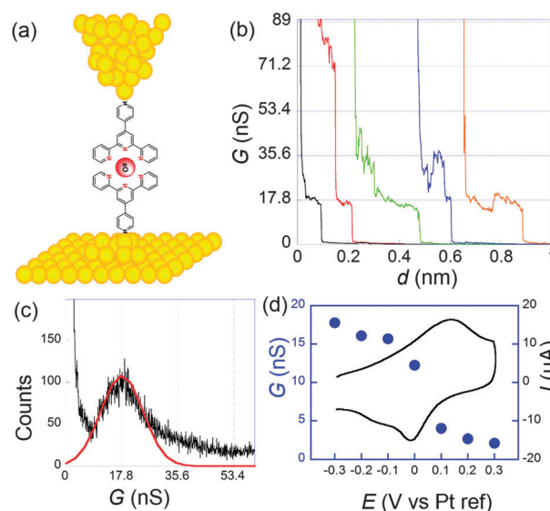
Fig. 4 (a) Schematization of a scanning tunneling microscopy break junction experiment. (b) A few conductance traces obtained for 1 at a sample potential of -0.3\text{ V} per Pt and a bias of 50\text{ mV} . Electrolyte: 0.1\text{ M NaClO}_4 aqueous solution. (c) Histogram obtained from the selection of 211 out of 1000 conductance traces. (d) Filled circles: molecular conductance versus sample potential. Black line: cyclic voltammogram. Adapted from ref. 45.
