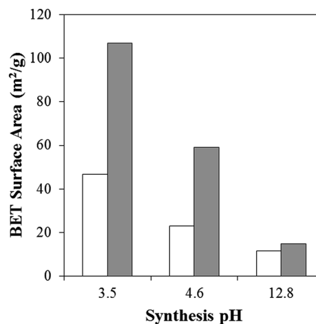
Fig. 7 BET specific surface area for boehmite (white) and alumina (grey) hydrothermally synthesised at pH 3.5, 4.6 and 12.8 for 20 h at 200 °C.
