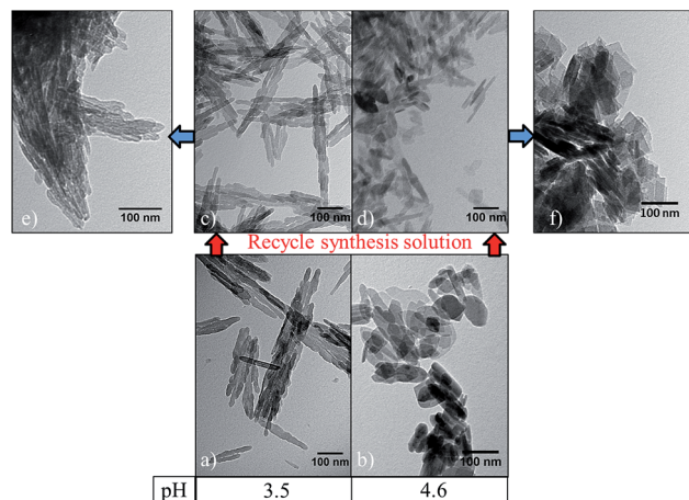
Fig. 4 Initial nanostructured \gamma\text{-AlOOH} hydrothermally synthesised ( 200^\circ\text{C} , 20 h) at (a) pH 3.5 and (b) 4.6 and morphology of \gamma\text{-AlOOH} synthesised by recycle procedure from initial pH (c) 3.5 and (d) 4.6. (e) and (f) show the morphology of resulting \gamma\text{-Al}_2\text{O}_3 samples after calcination of (c) and (d) respectively.
