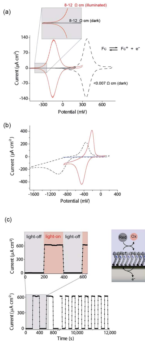
Fig. 2 (a) A cyclic voltammogram (CV) (dash black line) in aqueous 1.0 M \text{HClO}_4 at highly doped ( <0.007 \Omega \text{ cm} , dopant concentration, N_A, >8 \times 10^{18} \text{ cm}^{-3} ) p-Si electrodes that behave electrochemically similar to metals. A CV of a poorly doped n-Si electrode ( 8\text{--}12 \Omega \text{ cm} , N_D, \sim 4.5 \times 10^{14} \text{ cm}^{-3} ) in the dark (solid black line) and light (solid red line) at 642 nm, \sim 300 \text{ mW cm}^{-2} . (b) CVs (dash black line) at highly doped p-Si electrodes ( <0.003 \Omega \text{ cm} , dopant concentration, N_A \sim 1 \times 10^{19} \text{ cm}^{-3} ) and poorly doped p-Si electrode (substrate: 1\text{--}10 \Omega \text{ cm} , N_A, \sim 8 \times 10^{14} \text{ cm}^{-3} ; illumination: 642 nm, \sim 300 \text{ mW cm}^{-2} ) to a surface bound anthraquinone at pH 10.1 in the dark (solid blue line) and light (solid red line). (c) Amperometric trace demonstrating the switching on and off of heterogeneous catalysis promoted by surface-bound ferrocene from an n-Si electrode to an aqueous ferrocyanide solution. The n-Si electrode is poised at +0.2 \text{ V versus Ag|AgCl| } 3 \text{ M NaCl} and 1 mM ferrocyanide [\text{Fe}(\text{CN})_6]^{4-} in solution recycles the ferricinium back to ferrocene with modulation of the illumination (0.1 M \text{KNO}_3 at pH 7; substrate: 8\text{--}12 \Omega \text{ cm} ; illumination: 527 nm, \sim 1.77 \text{ mW cm}^{-2} , modulation is 200 s ON and 200 s OFF).
