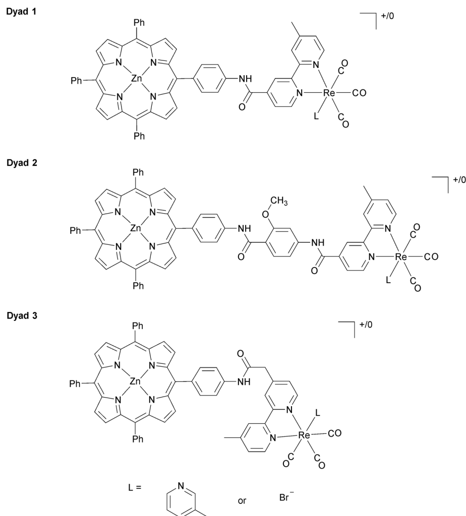
Fig. 1 Structure of Dyads 1–3. When L = 3-picolone, the dyads are positively charged, and labelled [Dyad 1 pic]PF 6 , [Dyad 2 pic]OTf, and [Dyad 3 pic]OTf. The Br complexes are neutral and are labelled Dyad 1 Br, Dyad 2 Br, and Dyad 3 Br.
