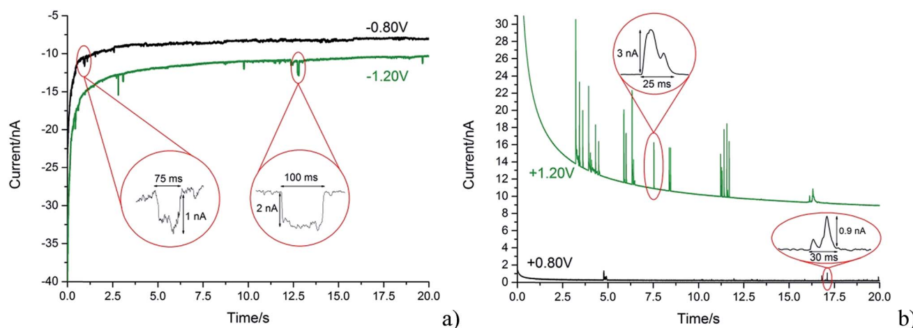
Fig. 5 Comparison of spike sizes at different potentials from representative chronoamperometric scans in a 5.9 \times 10^{-13} mol dm ^{-3} suspension using a cylindrical carbon fibre wire electrode. Smaller features at lower applied potential (vs. SCE) magnitude can be seen. (a) Black line: -0.80 V (vs. SCE). Green line: -1.20 V (vs. SCE). (b) Black line: +0.80 V (vs. SCE). Green line: +1.20 V (vs. SCE).
