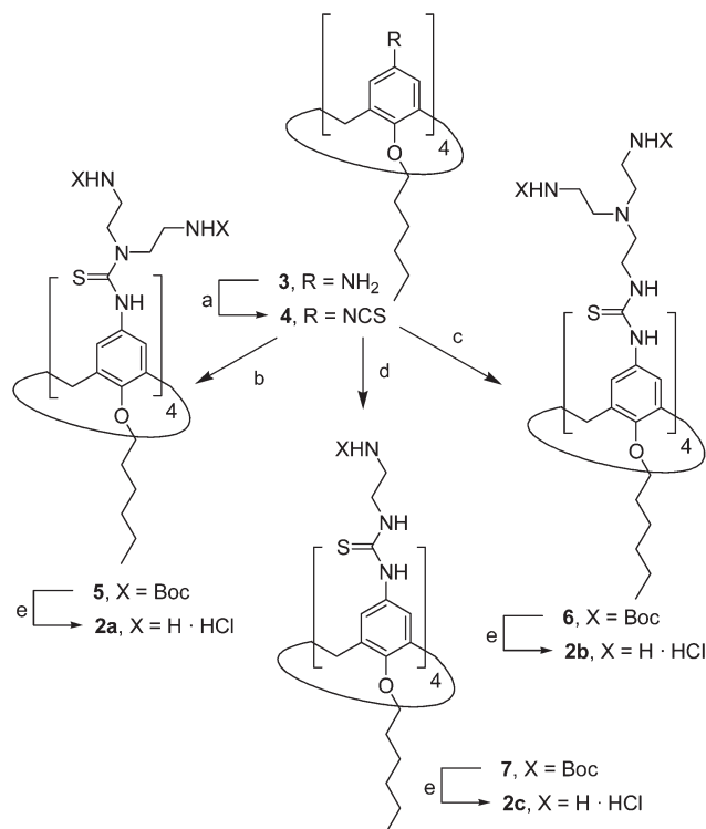
Scheme 1 Synthesis of polyaminothioureido CA_4 derivatives 2a–c . Reagents and conditions: (a) (i) CS_2 , Et_3N , EtOH , rt, 2 h; (ii) Boc_2O , DMAP, EtOH , 0\text{ }^\circ C \rightarrow rt , 2 h, 88%; (b) NH(CH_2CH_2NHBoc)_2 , Et_3N , DCM, rt, 12 h, quantitative; (c) H_2NCH_2CH_2N(CH_2CH_2NHBoc)_2 , Et_3N , DCM, rt, 12 h, 99%; (d) NH_2CH_2CH_2NHBoc , Et_3N , DCM, rt, 1.2 h, 99%; (e) (i) TFA–TES–DCM, 5 min, rt; (ii) HCl, 99%.
