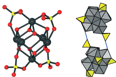
In addition, four carboxylate groups of the organic linker molecules are coordinating in the equatorial plane of the cluster, leading to a square grid layer based on inorganic nodes
