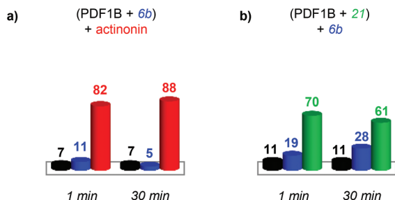
Fig. 7 Indirect sequential competition experiments monitored by real-time ion-mobility mass spectrometry. Relative proportions, calculated from the arrival time distribution intensities of the 9+ and 8+ charge states, of apoPDF1B (black), PDF1B : actinonin (red), PDF1B : 21 (green) and PDF1B : 6b (blue) 1 and 30 min after adding the second ligand in sequential incubations of (a) 6b and then actinonin and (b) 21 and then 6b.
