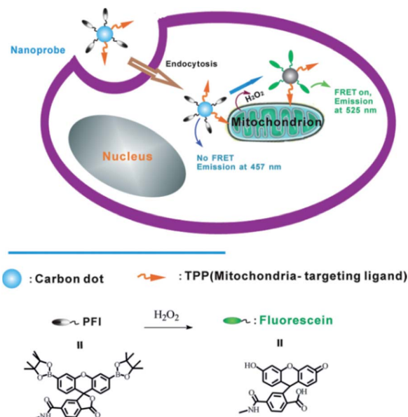
Fig. 23 Schematic illustration of FRET-based ratiometric sensing of mitochondrial \text{H}_2\text{O}_2 in living cells by the nanoprobe. Adapted with permission. 110 Copyright 2014, Wiley-VCH.
