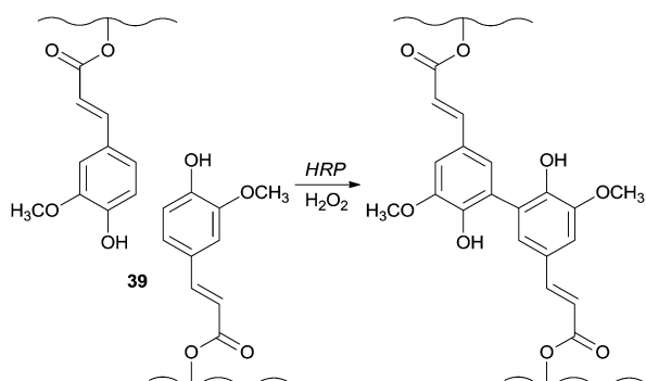
Scheme 10 Formation of in situ gellable sugar beet pectin (SBP).
