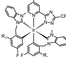
55: \text{R}_1 = \text{H} , \text{R}_2 = \text{'Bu} (\text{fbmb})_2\text{Ir}(\text{bptz})
