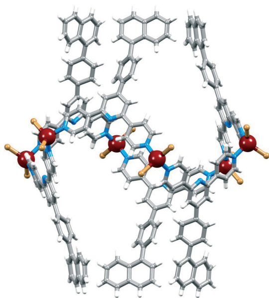
Fig. 8 Structure of the centrosymmetric [\{\text{ZnBr}_2(3)\}_6] molecule in [\{\text{ZnBr}_2(3)\}_6] \cdot 3\text{CHCl}_3 \cdot 15\text{H}_2\text{O} ; the metallohexacycle adopts conformer I.
