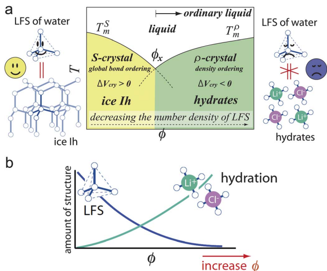
Fig. 30 (a) Schematic phase diagram of water–LiCl mixtures. 228 Locally favoured structures have a symmetry consistent with ice crystals ( S -crystal), but not with hydrate crystals ( p -crystal). In this figure, if we replace the salt concentration \phi by pressure, it represents the phase diagram of water or other water-type liquids. Although both addition of salt and application of pressure leads to the decrease in locally favoured tetrahedral structures, their roles should have some difference since the former has local effects whereas the latter has global effects. (b) Schematic representation of the \phi dependence of the fraction of locally favoured structures and hydration structures. Note that locally favoured structures are the source of frustration against hydrate crystals ( p -crystal). This figure is courtesy of Mika Kobayashi.
