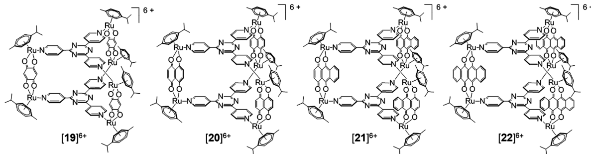
Chart 9 Molecular structures of metalla-cages [19] 6+ , [20] 6+ , [21] 6+ , and [22] 6+ .
