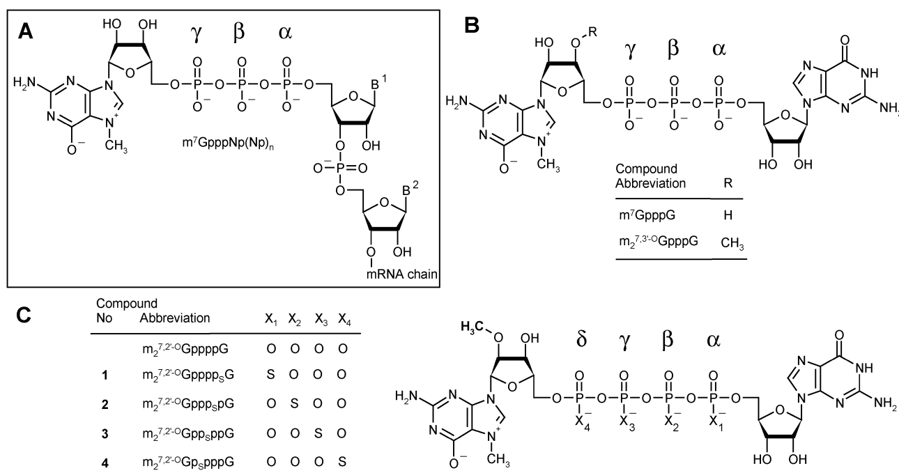
Fig. 1 Cap structures. (A) A general depiction of the eukaryotic mRNA 5'-end. (B) Structures of standard triphosphate analogs: m 7 GpppG and m 2 7,3'-O GpppG (ARCA). (C) Structures of m 2 7,2'-O GpppG and analogs synthesized in this study.
