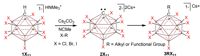
Figure 1. Synthesis of C-functionalized [\text{RCB}_{11}\text{X}_{11}]^{1-} anions 3RX 11 with \text{Cs}_2\text{CO}_3 .
