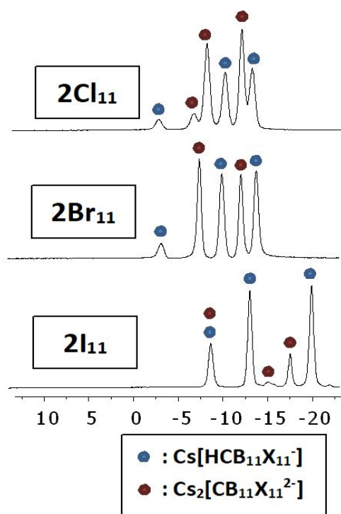
Figure 2. \text{HNMe}_3^+ salts of 1X 11 reacted with 2 eq of \text{Cs}_2\text{CO}_3 yields equilibrium mixtures of 1X 11 and 2X 11 .
