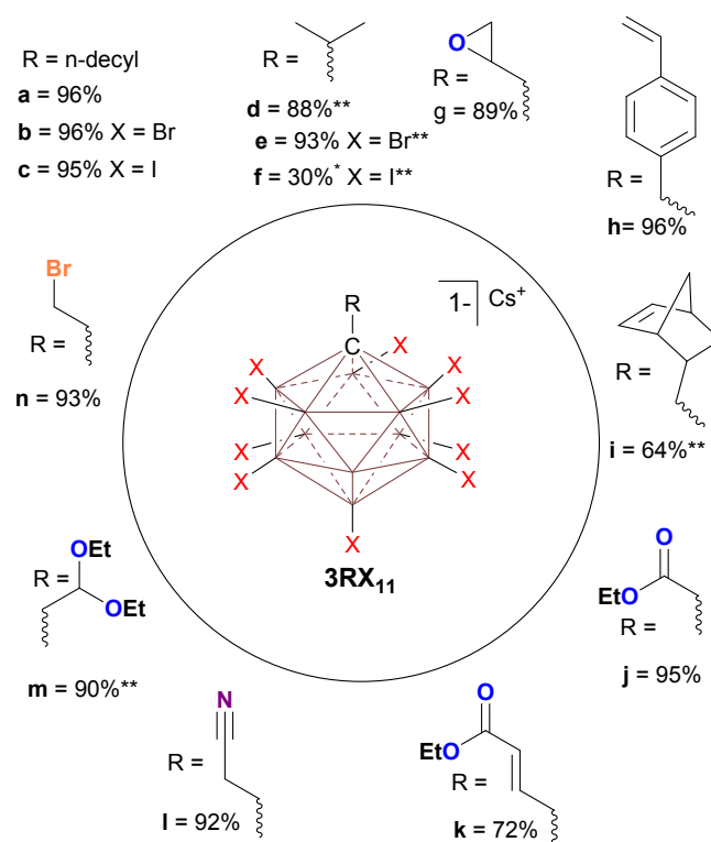
Figure 3. Scope of cesium carbonate mediated C-H functionalization of [\text{HCB}_{11}\text{X}_{11}^{-1}] cages 1 . Yields were calculated by weighing the purified salt products. * = conversion via NMR not isolated yield; reactions were performed at room temperature unless indicated by ** (= 85 °C). Unlabeled vertices = B.
