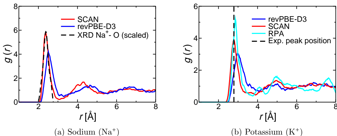
Figure 2: RDFs of solvated sodium and potassium ions in water with the revPBE-D3 and SCAN functionals demonstrating that the SCAN functional reproduces the experimentally observed peak position ( \text{Na}^+ , \text{K}^+ ) and peak shape ( \text{Na}^+ ) much more accurately.
