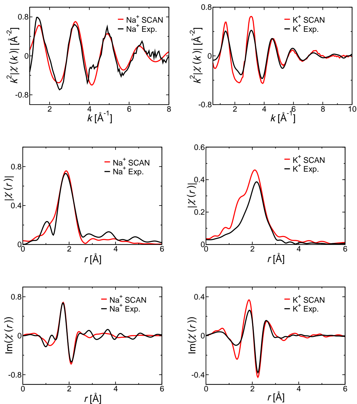
Figure 5: EXAFS calculations compared with experiment for sodium (left) and potassium (right). Experimental data for potassium is from Ref. 58 . Experimental data for sodium is from Ref. 20 after revision for self-absorption (see Experimental Details).
