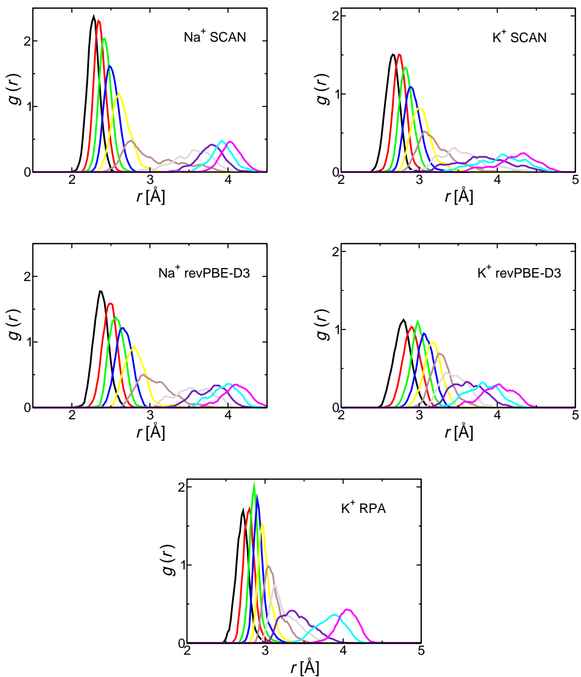
Figure 3: Incremental RDFs of the sodium and potassium ions in water with the SCAN, revPBE-D3 and RPA functional. Black gives the distribution of the closest molecule, red the second closest etc.
