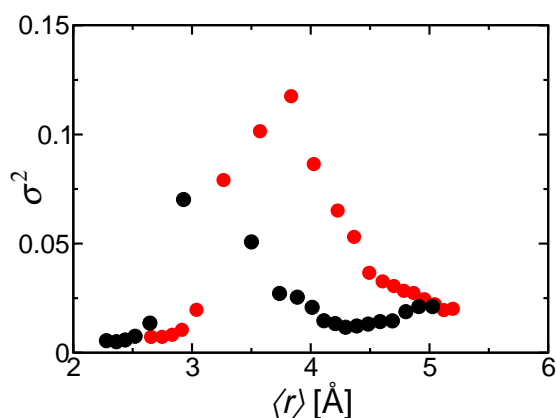
Figure 4: Analysis of the incremental RDFs for sodium (black) and potassium (red) with the SCAN functional. Each point gives the average position and fluctuation in the position (the Debye-Waller factor) of one water molecule in the incremental RDF.
