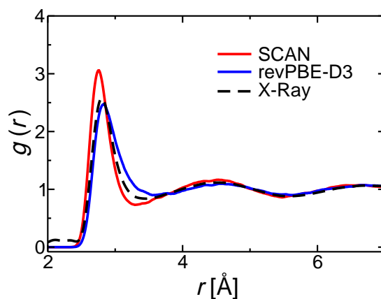
Figure 1: Oxygen-oxygen RDFs with the revPBE-D3 and SCAN functionals compared with experimental XRD data. 45
