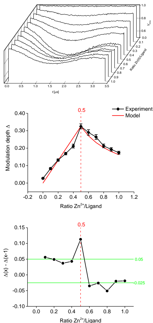
Fig. 3: Top Waterfall plot of the background-corrected PELDOR traces. Middle Experimental ( \pm RMSD) and modelled modulation depth. Bottom Respective changes in mean modulation depth in relation to the metal-nitroxide ratio.
