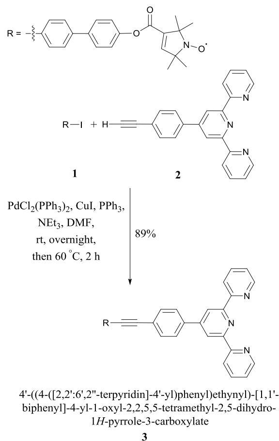
Scheme 1: Synthesis of the tpy-based ligand (tpyNO).
