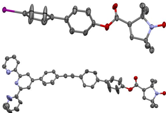
Fig. 1: Crystal structures of compounds 1 (top) and 3 (bottom). Displacement ellipsoids are drawn at 50% probability; hydrogen atoms, solvent molecules, and minor components of the disorder are omitted for clarity.
