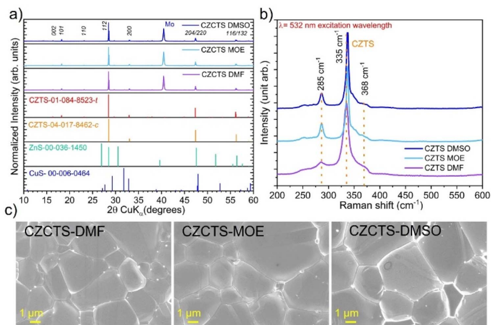
Fig. 1 (a) X-ray diffraction, (b) Raman spectroscopy, (c) top-view SEM images of CZTS films elaborated using different solvents.
