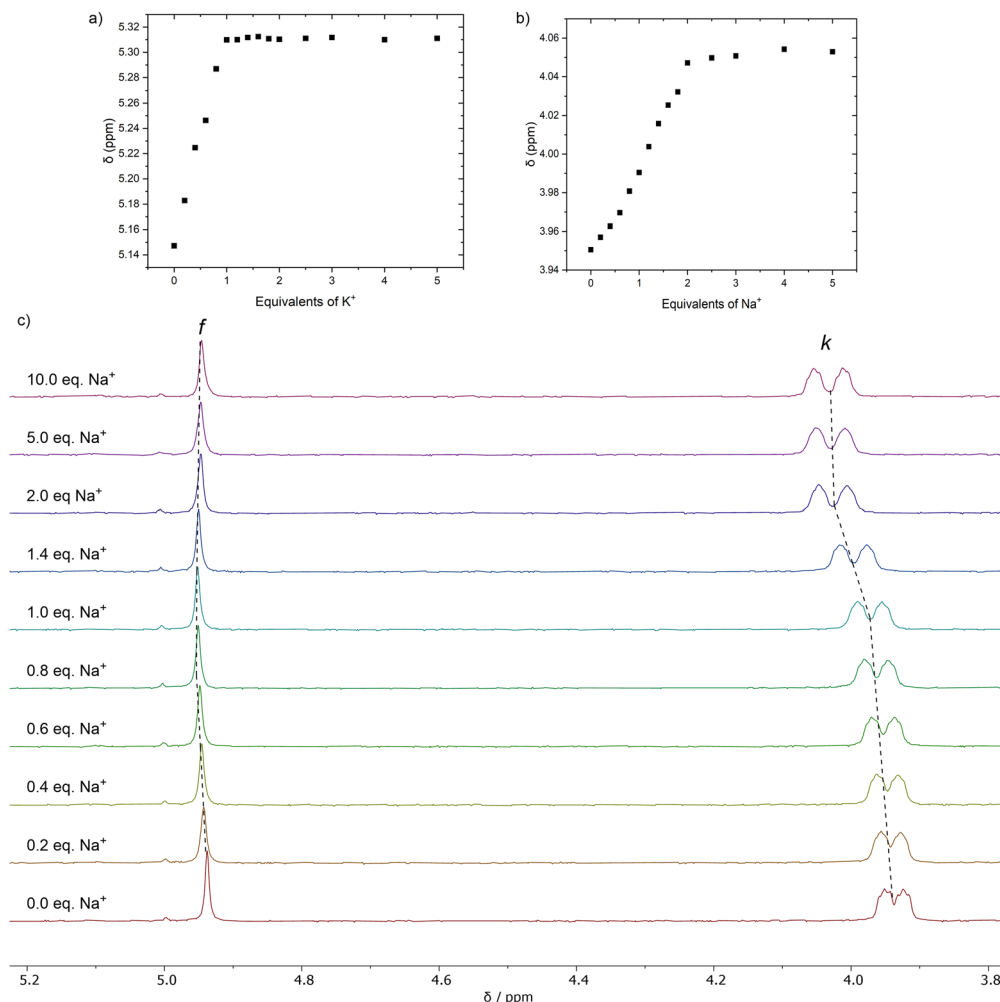
Fig. 3 (a) Binding isotherm showing ^1\text{H} NMR (500 MHz, 298 K, 1:1 v/v \text{CDCl}_3 : \text{CD}_3\text{CN} ) resonance of proton H_f of 6-Ni upon sequential addition of \text{KBAR}_4^{\text{F}_4} solution. (b) Binding isotherm showing ^1\text{H} NMR (500 MHz, 298 K, 1:1 v/v \text{CDCl}_3 : \text{CD}_3\text{CN} ) resonance of proton H_k of 6-Ni upon sequential addition of \text{NaBAR}_4^{\text{F}_4} solution. (c) Stacked partial ^1\text{H} NMR (500 MHz, 298 K, 1:1 v/v \text{CDCl}_3 : \text{CD}_3\text{CN} ) spectra of 6-Ni upon sequential addition of \text{NaBAR}_4^{\text{F}_4} solution.
