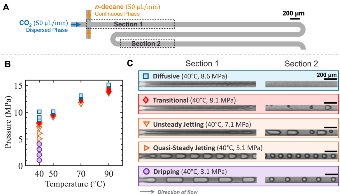
Fig. 2 (A) Microchannel schematic showing section 1 and section 2 as the regions of interest under a microscope with a 10 \times objective. CO 2 (dispersed phase) and n -decane (continuous phase) were co-injected at a constant flow rate of 50 \mu\text{L min}^{-1} at the flow-focusing junction. Section 1 captures the junction where the CO 2 -decane interface forms, while section 2 is located downstream (8.6 mm from the junction). (B) Phase diagram summarizing all the experimental conditions, showing flow regime transitions at T = 40, 50, 70, and 90 ^{\circ}\text{C} . (C) Representative snapshots at T = 40 ^{\circ}\text{C} for each flow regime, captured from section 1 (left) and section 2 (right) as indicated in (A). Experimental conditions are noted; scale bars: 200 \mu\text{m} .
