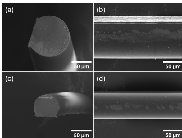
Fig. 1 SEM images of air-dried as-spun Kraft lignin–PVA fibres spun continuously from [DMBA][HSO 4 ] and water mixtures using a 25 G (260 \mu m) spinneret (a and b) and a 30 G (159 \mu m) spinneret (c and d).
