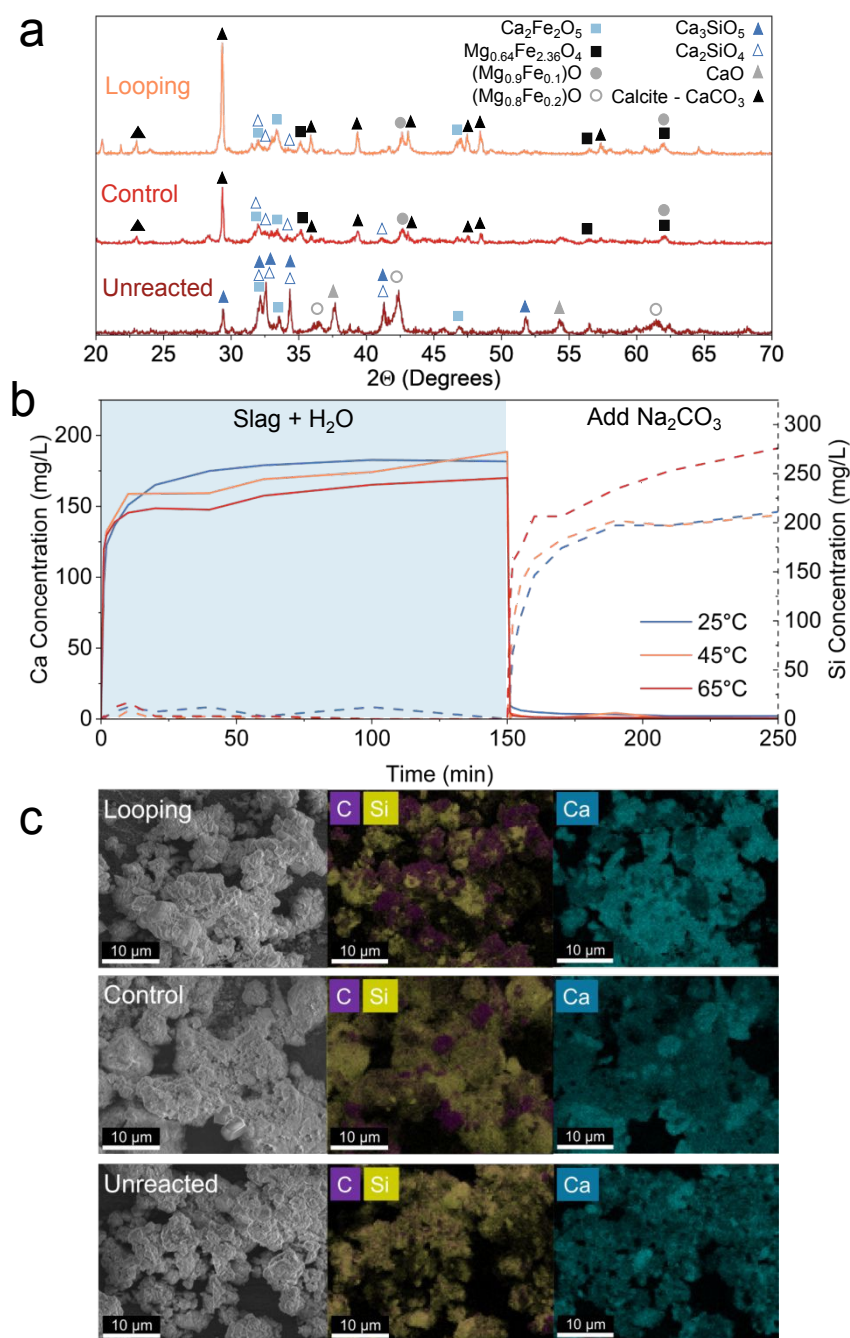
Fig. 6 (a) X-ray diffraction (XRD) comparing unreacted quenched BOF slag with slags after the control process and after Na 2 CO 3 looping process, each process including 10 cycles with 4% CO 2 at 45°C. (b) Calcium (Ca) and silicon (Si) concentration evolution in aqueous solution during hydration of quenched slag in water, followed by addition of Na 2 CO 3 . (c) Scanning Electron Microscopy (SEM) and Energy Dispersive X-Ray Spectroscopy (EDS) maps to compare the distribution of Ca, Si, and carbon (C) in unreacted quenched BOF slag with slags after the control process and after Na 2 CO 3 looping process, each process including 10 cycles with 4% CO 2 at 45°C. XRD and elemental mapping show a higher degree of CO 2 mineralization by Na 2 CO 3 looping than the control process.
