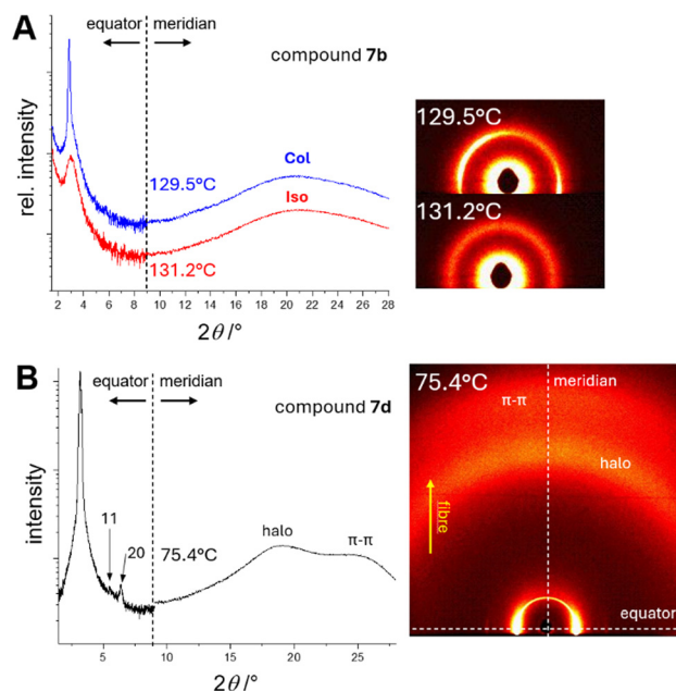
Fig. 5 (A) Diffraction pattern of 7b with integrated intensity of the equator and meridian. (B) Diffraction pattern of 7d at 75.4 °C with integrated intensities and assigned miller indices.
